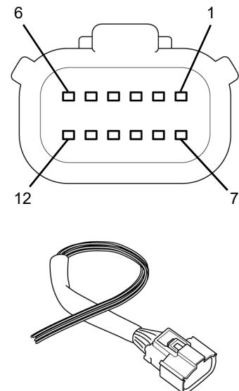
Molex MX150 12-poles connector, cable view and wire harness (optional components manufactured by Veratron)
