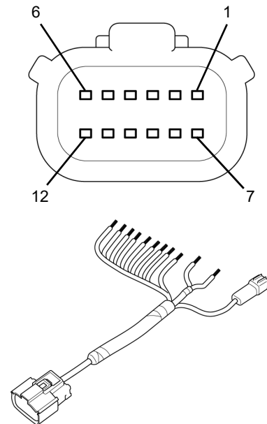
Molex MX150 12-poles connector, cable view and wire harness (included)
