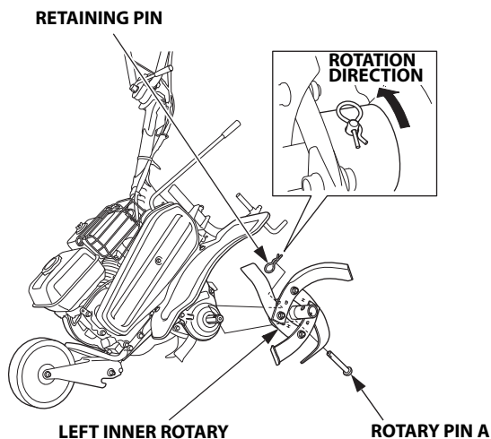
ROTARY PIN A (LONG)
