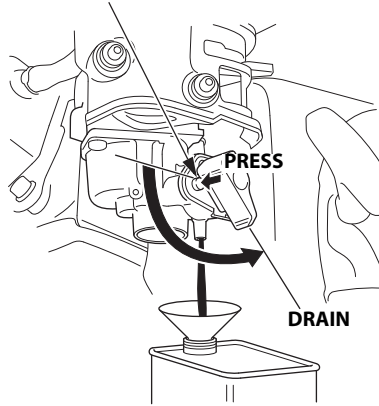
STOPPER BUTTON
