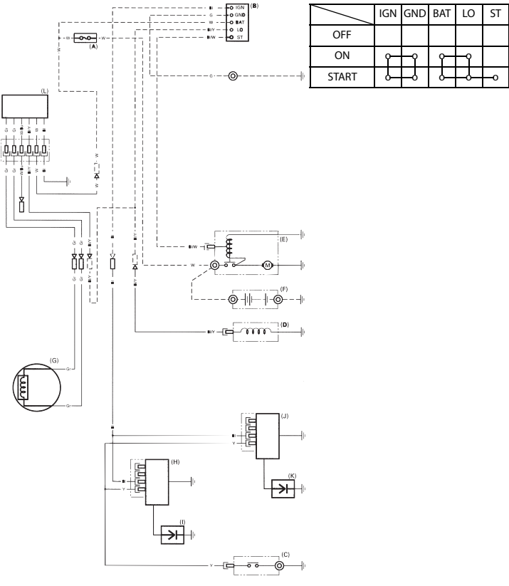
17 A Charge Coil and Without Control Box Type
