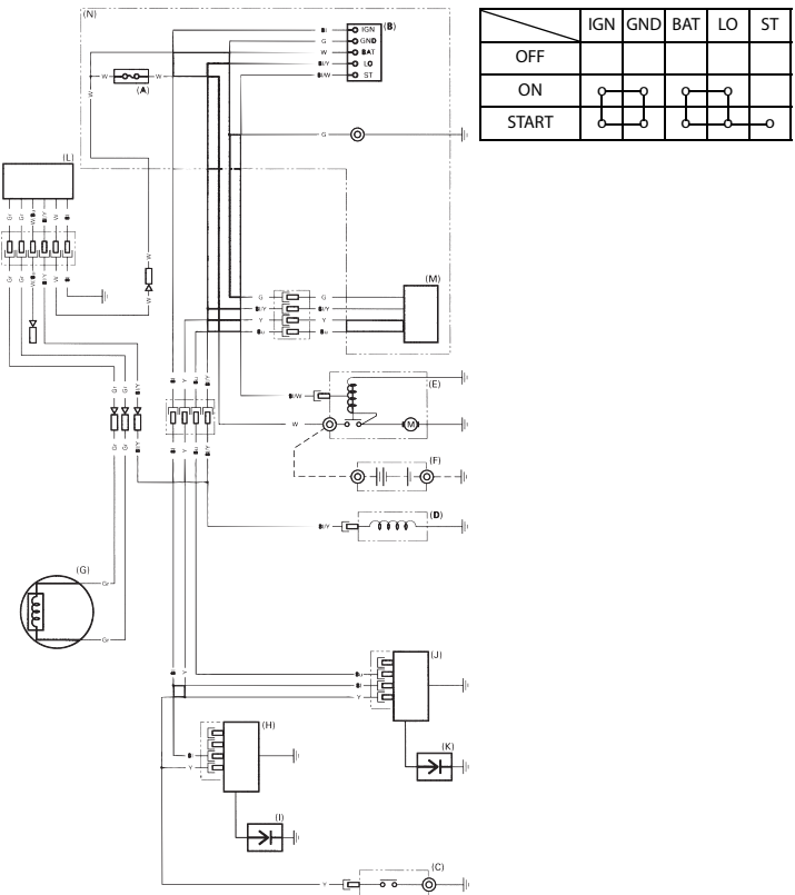
17 A Charge Coil and With Control Box Type
