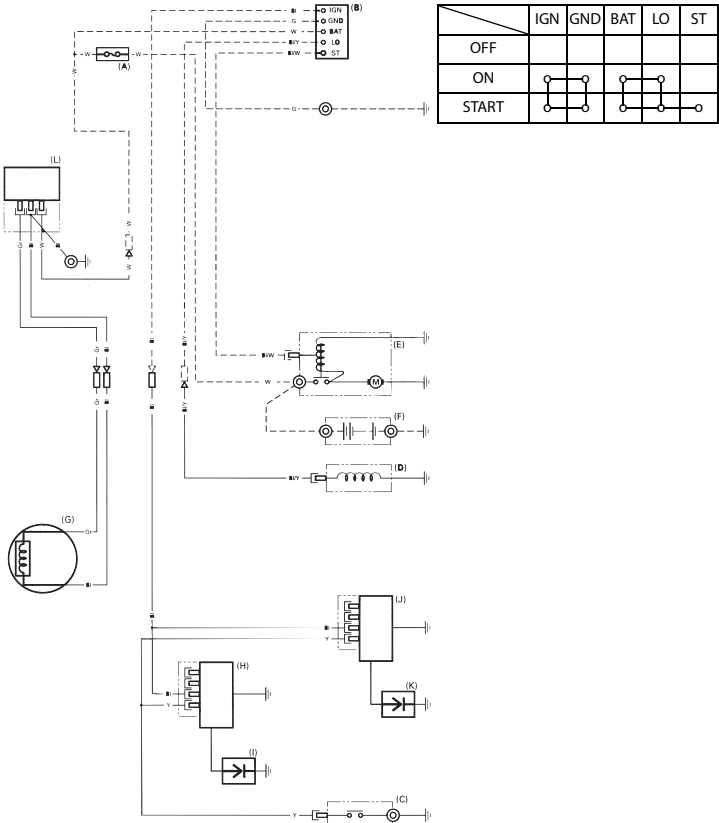
2.7 A Charge Coil and Without Control Box Type
