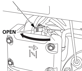
CHOKE LEVER
